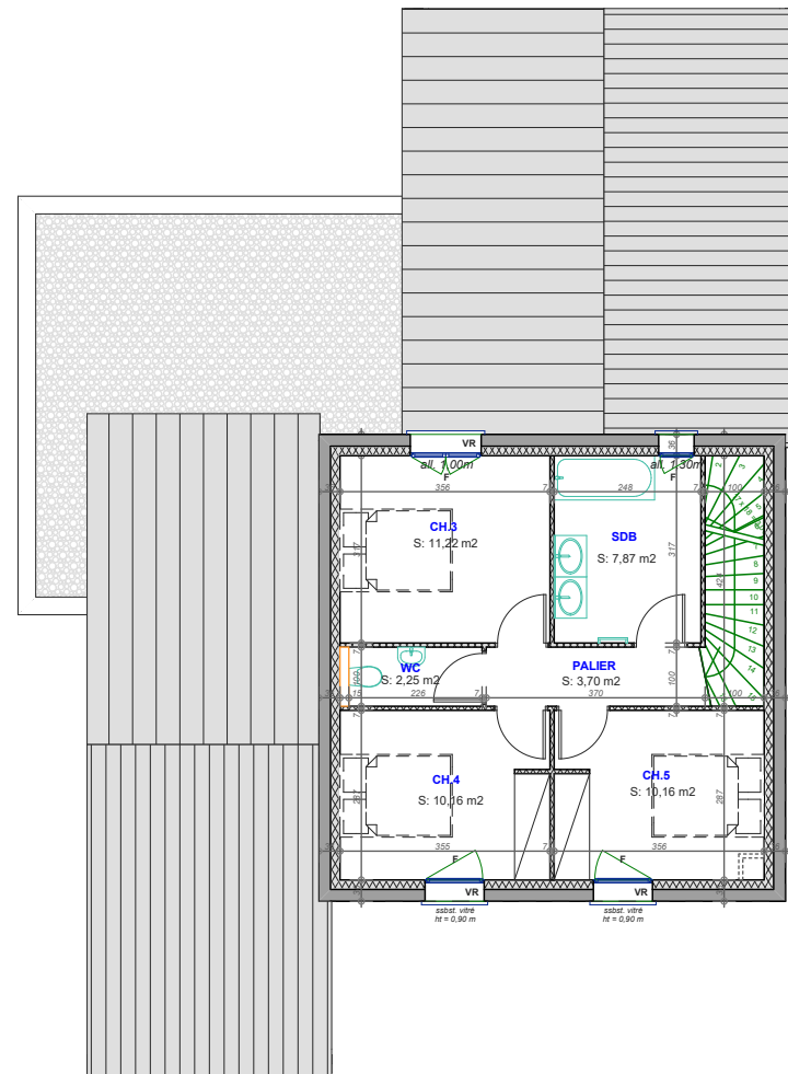
Plan R+1
